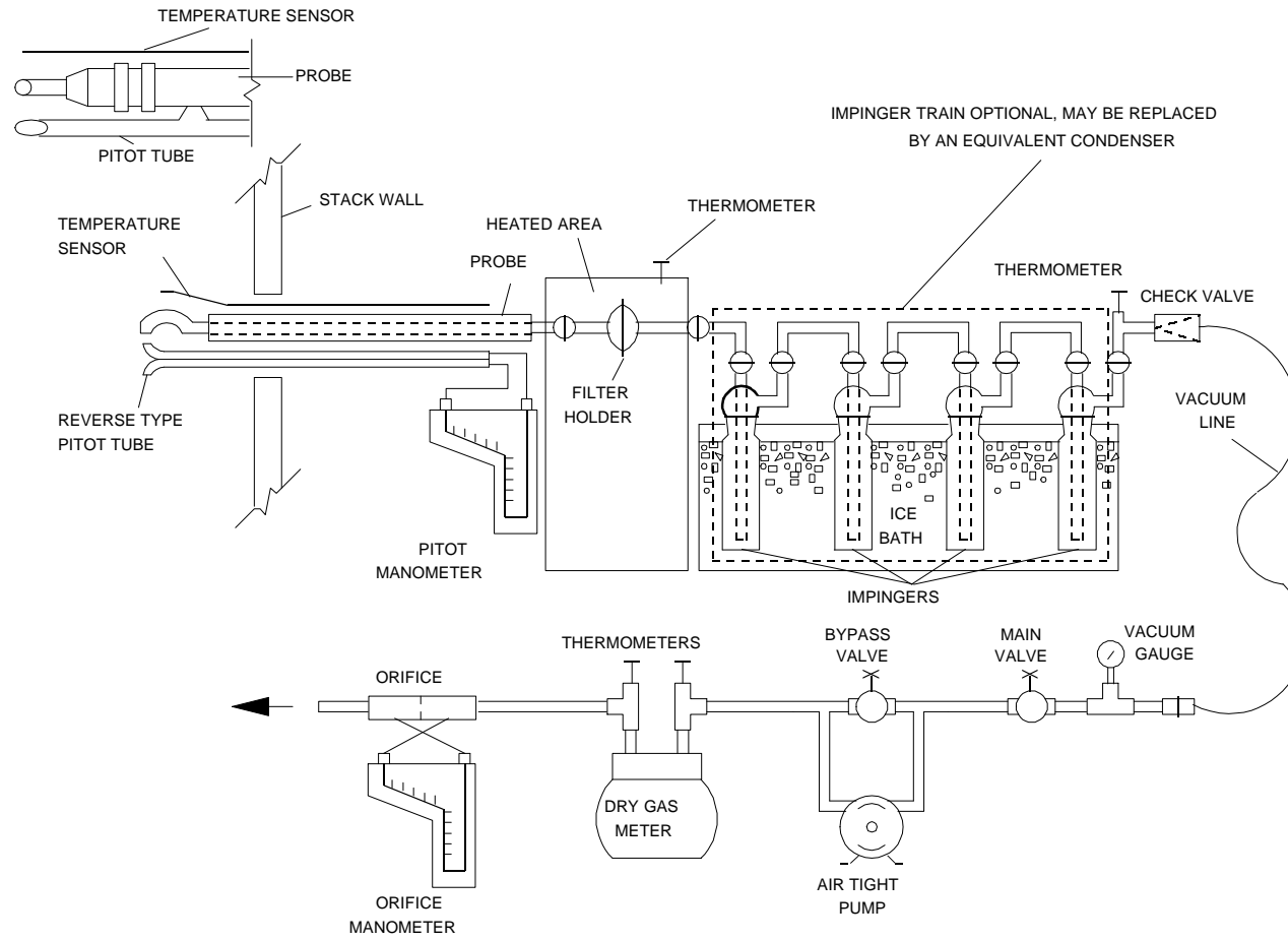
Figure 5-1. Particulate Sampling Train
