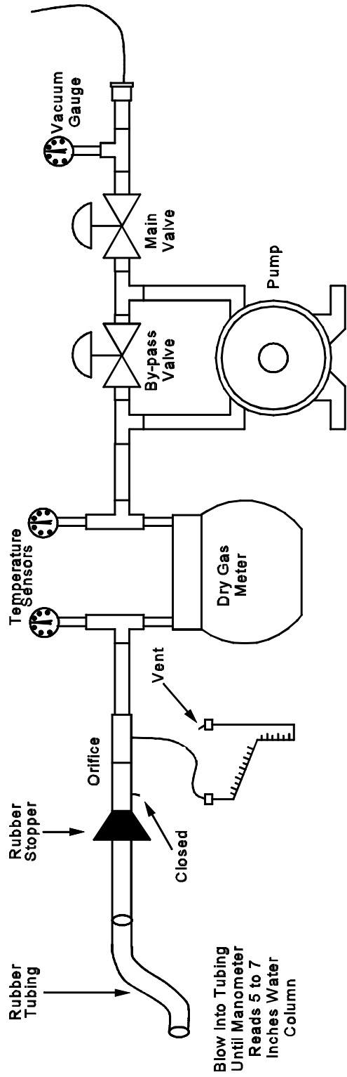
Figure 5-4. Leak Check of Meter Box.
